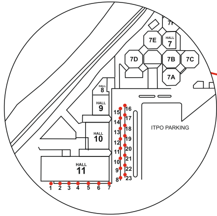
POLE LOCATION & NOS.
